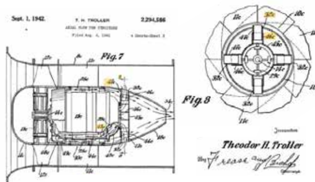
Dr. Theodor H. Troller held numerous patents including the one above for the Axial Flow Fan Structure he invented.
